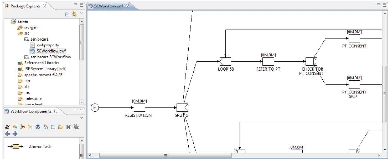
Fig 1.6: SCWorkflow.cwf
